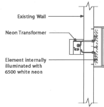
Elevation n-Side/Section
